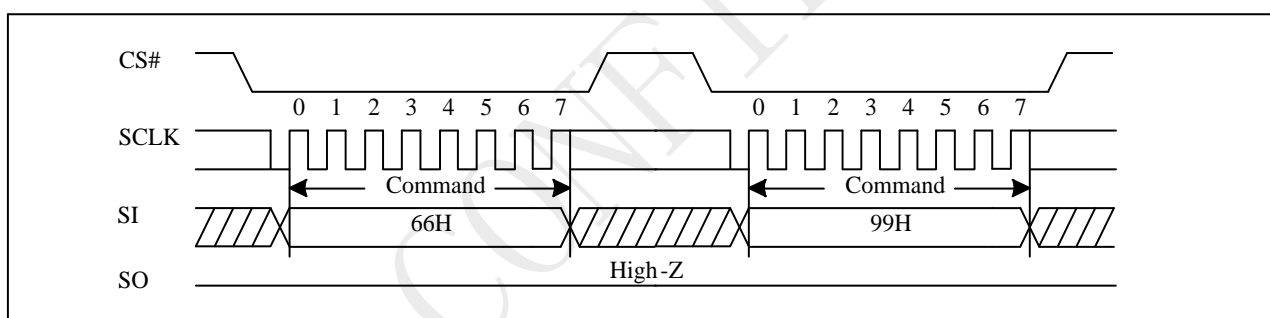
Figure 10-57b Reset Sequence(QPI)
