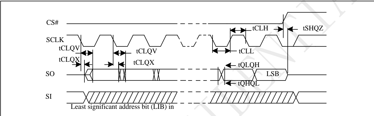
Figure 5-6 Hold Timing
