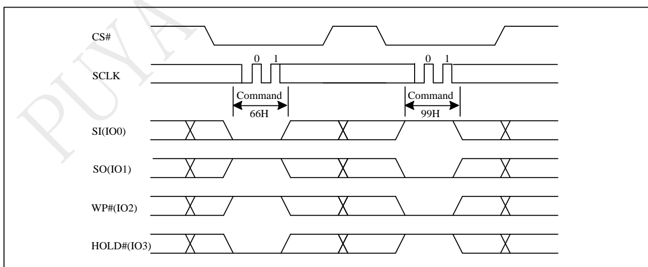
Figure 10-57b Reset Sequence(QPI)
