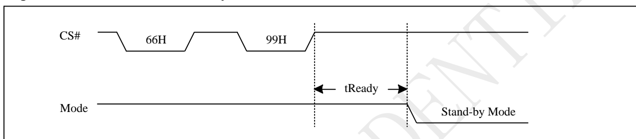
Figure 10-57a Reset Sequence
